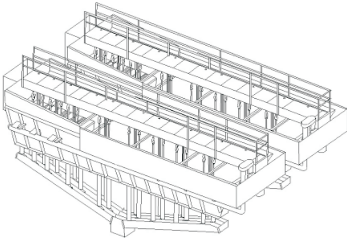
Classifying Tanks - the simplest way to truly "Classify" and reblend
